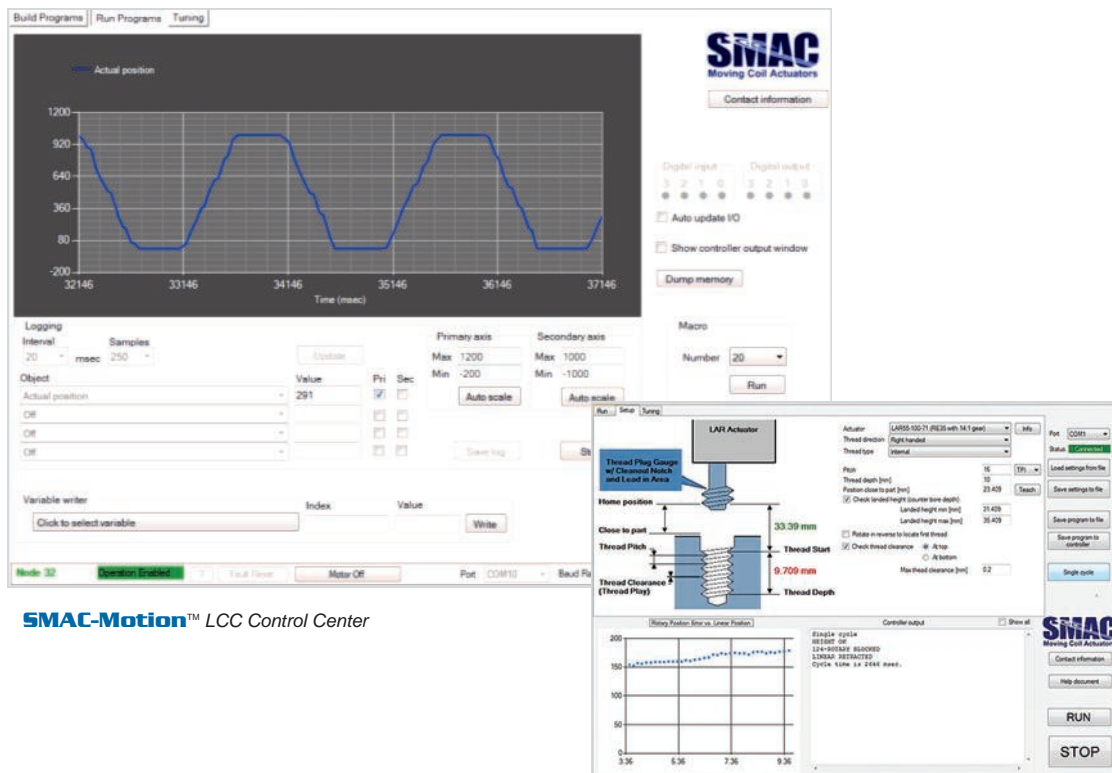
SMAC-Motion™ Thread Check
